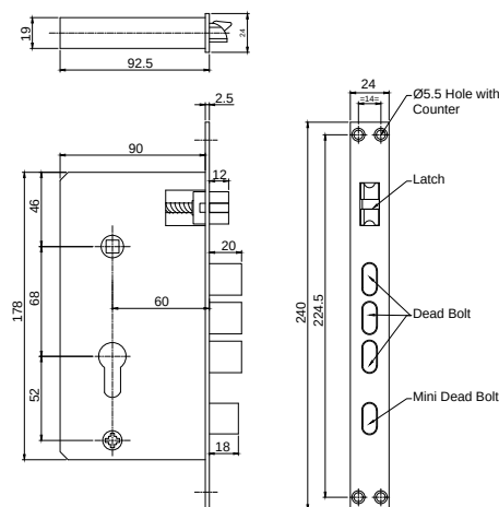
60 x 68mm Lock Body
