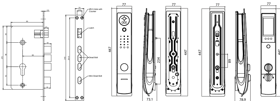
60 x 68mm Lock Body
