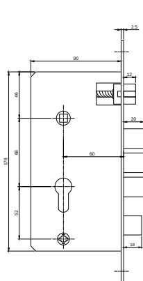
60 x 68mm Lock Body
