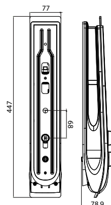
Back Panel
